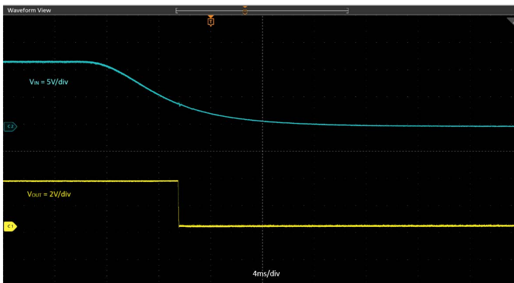
Figure 5: MxL76502 Shutdown with a 2A Load
