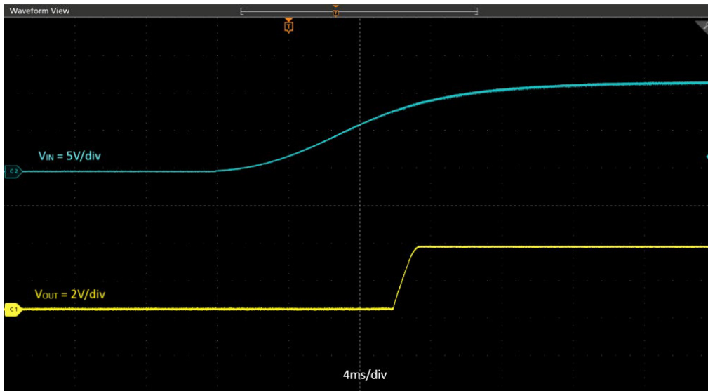
Figure 4: MxL76502 Start-Up with a 2A Load
