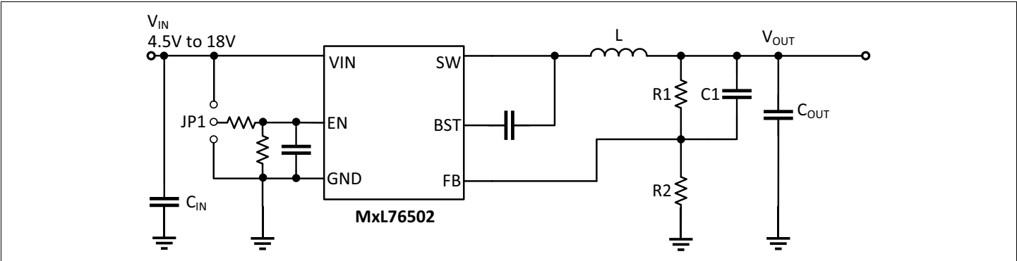
Figure 2: MxL76502 EVK Simplified Block Diagram
