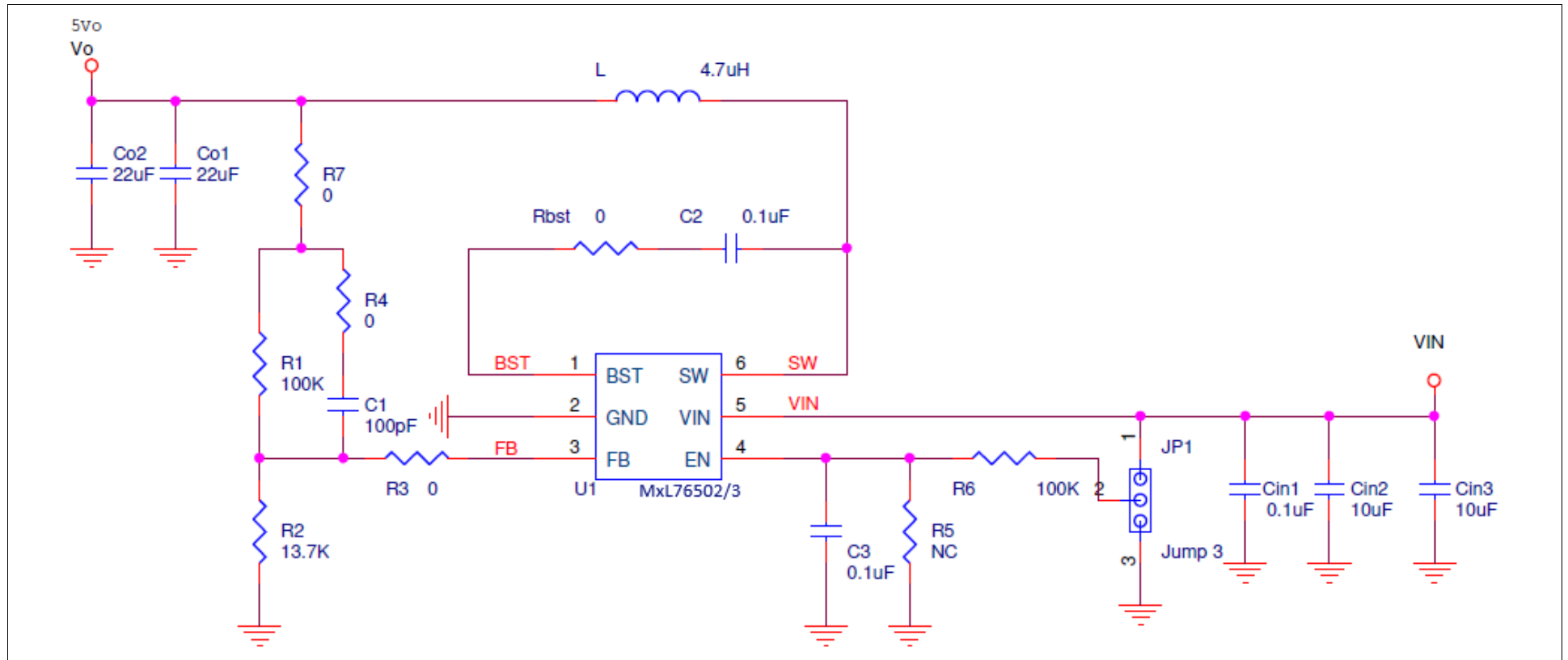
Figure 6: EVK Schematic
